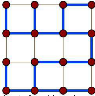
A spanning tree (blue heavy edges) of a grid graph. Spanning forests
