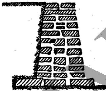
Fig 11.10 Dry Rubble Masonry
