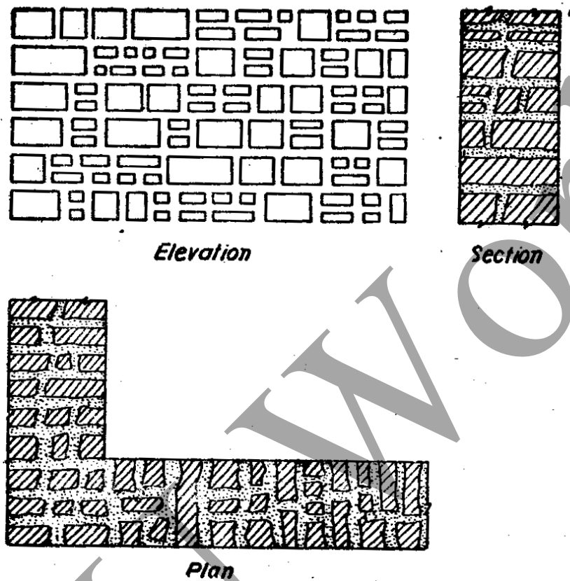
Fig 11.6 Coursed Squared Rubble Masonry
