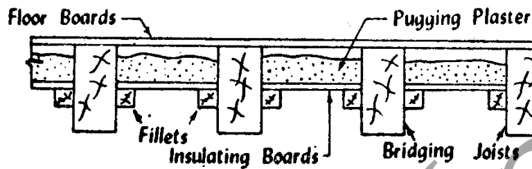
Fig 12.1 Pugging
