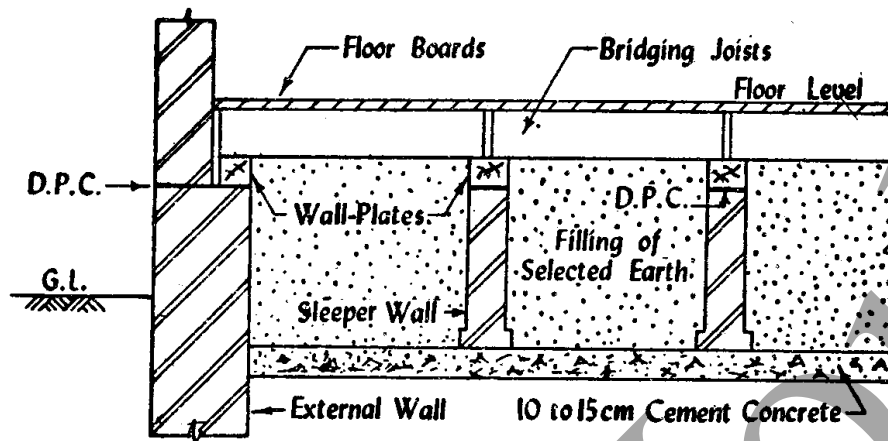
Fig 12.2. Basement or ground floor of timber
