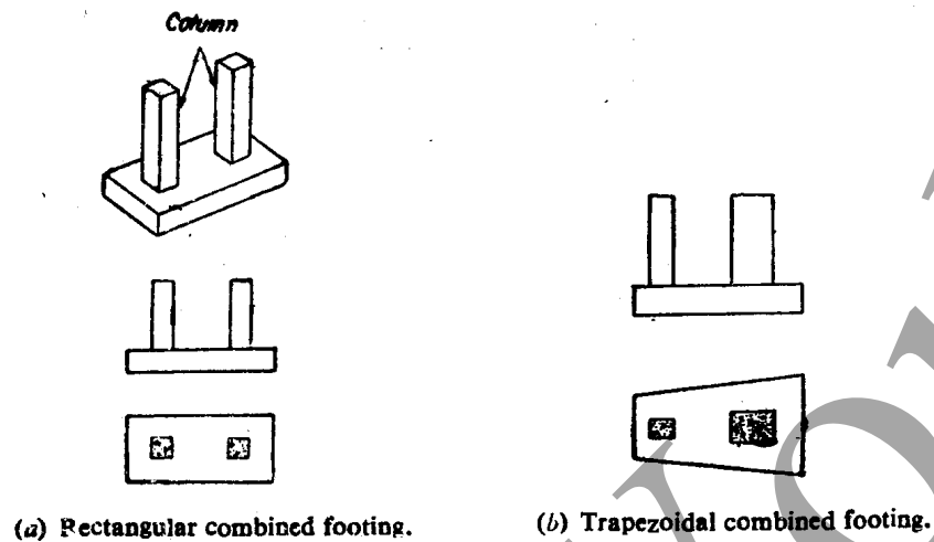
Fig 10.5 Combined Footings
