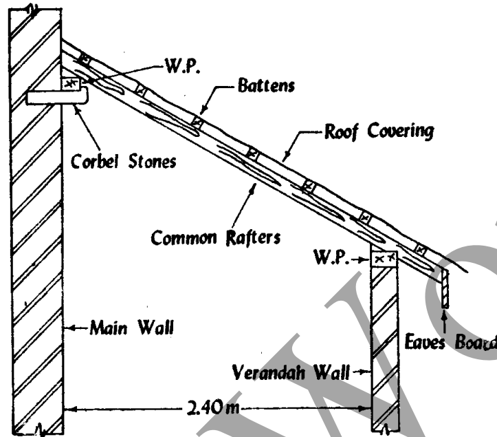
Fig 13.3 Lean-to roof
