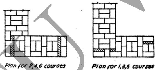
Two-bricks double flemish bond.
