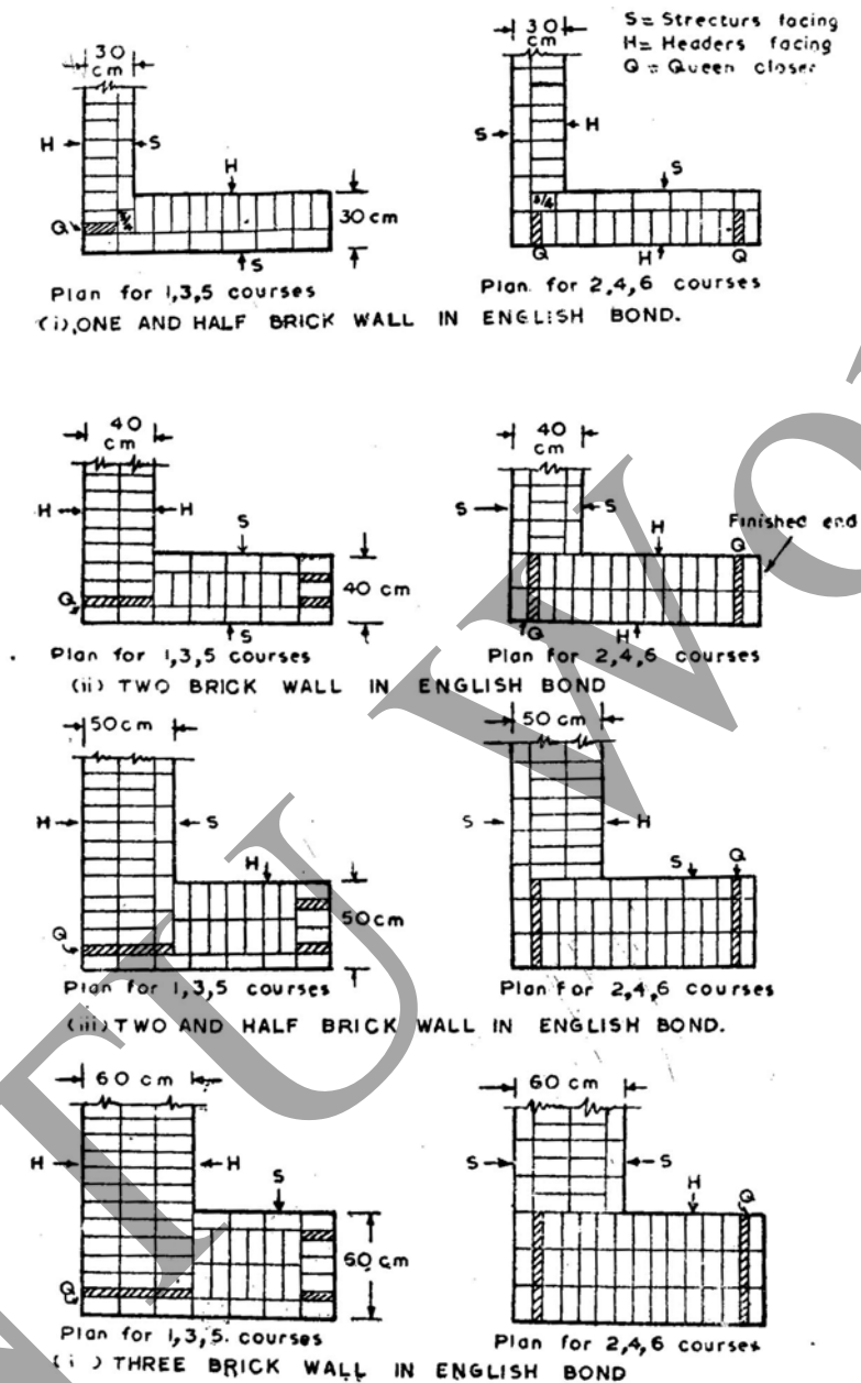
Fig 11.17 Alternate arrangements for various wall thicknesses in English Bond
