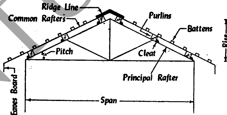
Fig 13.2 Truss
