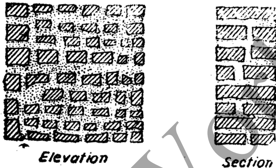
Fig 11.3 Uncoursed random rubble masonry
