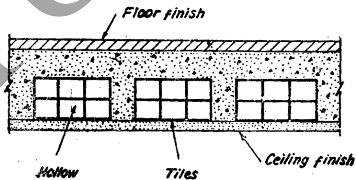
Fire-resisting—Hollow tiled Ribbed floor.
